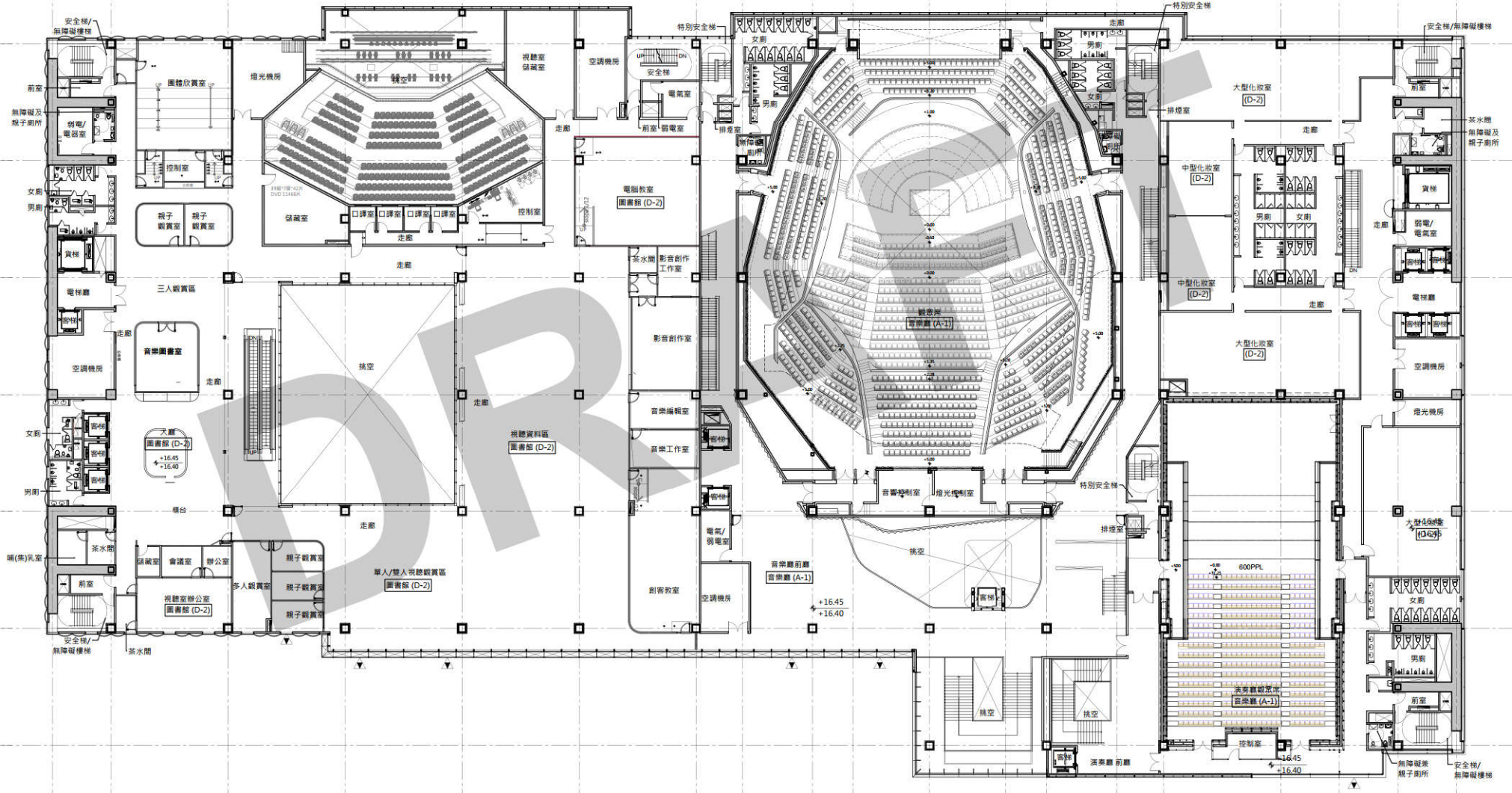
4F PLAN
